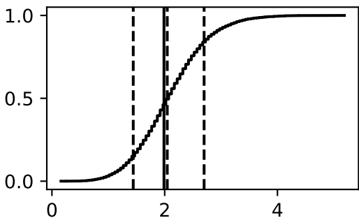
CDFs of c_0 , c_1 , and c_2
