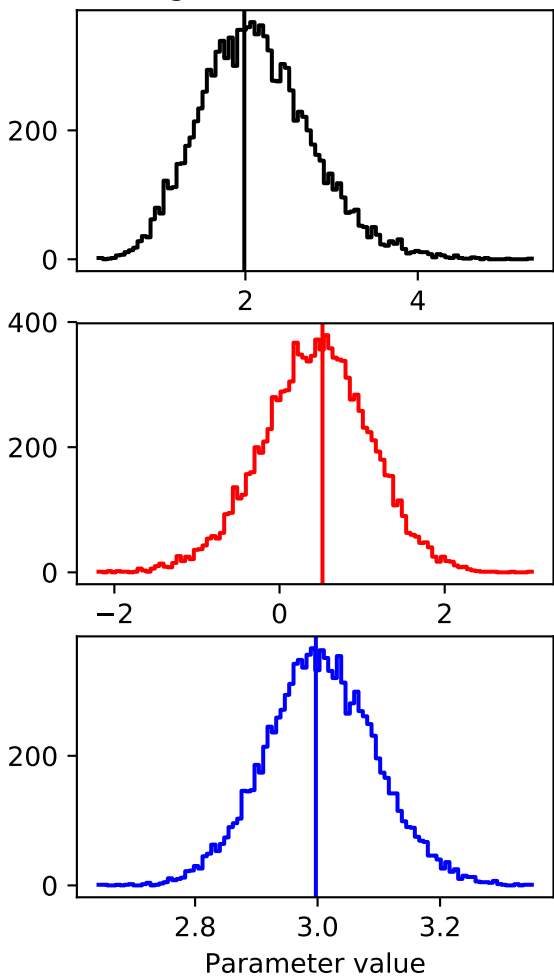
Histograms of c_0 , c_1 , and c_2
