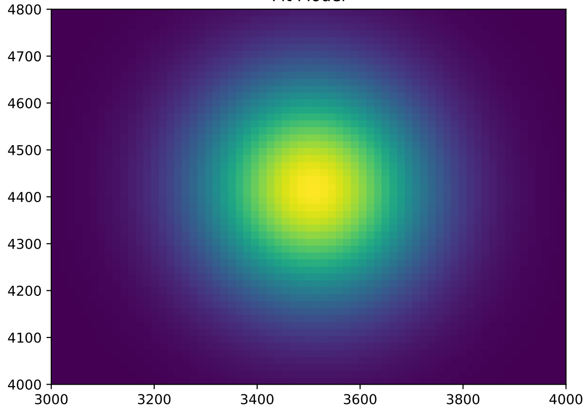
Fit Model
