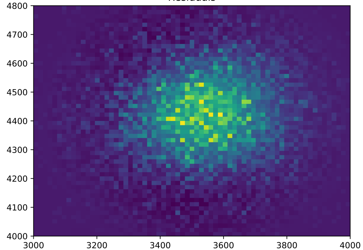
Residuals
